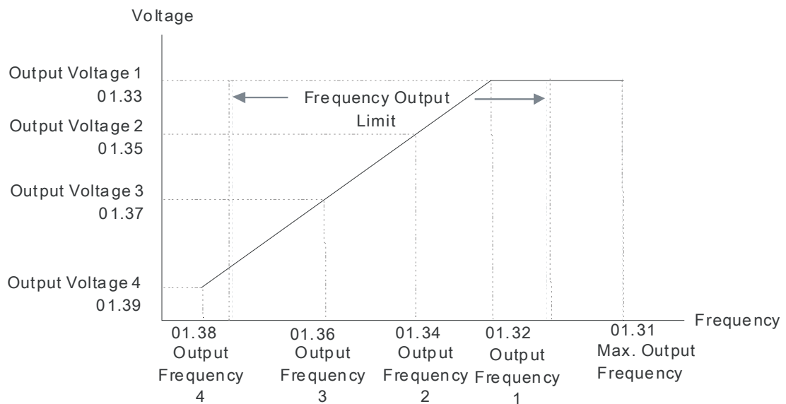
V/F Curve
